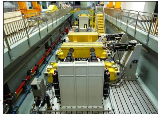
Vibration test machine
